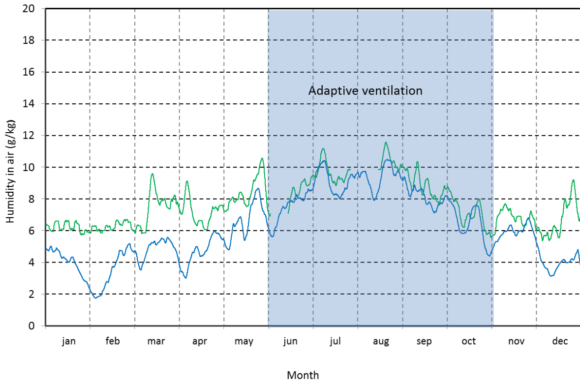
Figure 5 The mixing ratio of the inside air (green) and outside air (blue) in Nødebo Church shown as a moving average over 7 days. The inside MR is higher than outside in winter, but equal in summer due to the ventilation.
