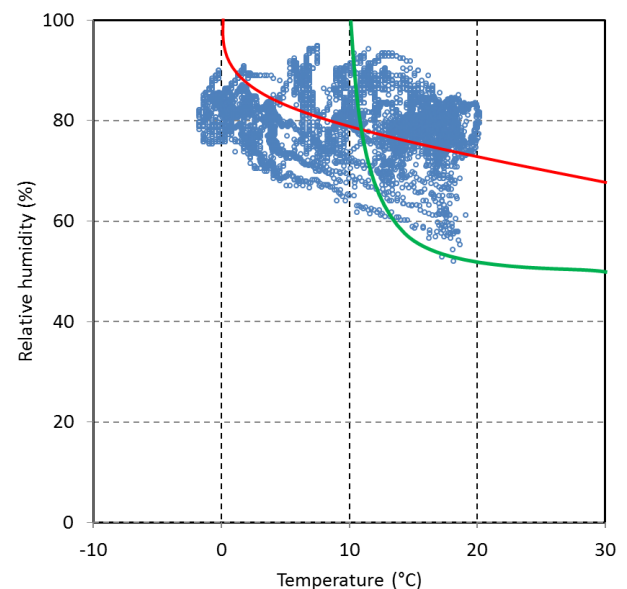
Figure 7 . Climate record in Tyvelse Church with basic heating in winter (above) and adaptive ventilation (below). Data periods are 1 September 2006 – 31 August 2007 and 1 June 2011 – 31. May 2012. Limits for mold growth (red line) and wood worms (green line)
