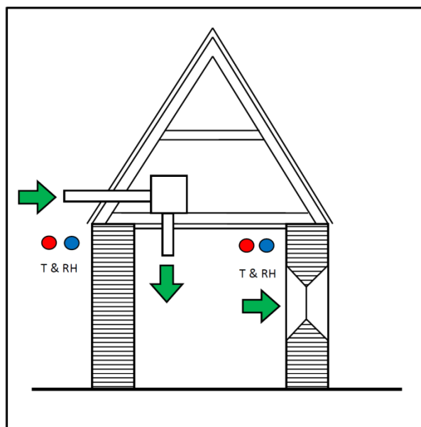
Figure 1 Principal diagram of a system for adaptive ventilation. The operation of the fan is controlled by a small computer connected to the inside and outside sensors for temperature and relative humidity.
