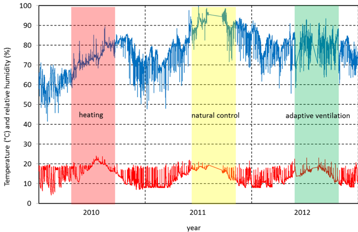
Figure 3 Climate record from Nødebo Church over three years. The first summer had heating to keep the RH below 80%. The next summer had no control and the last summer had adaptive ventilation
