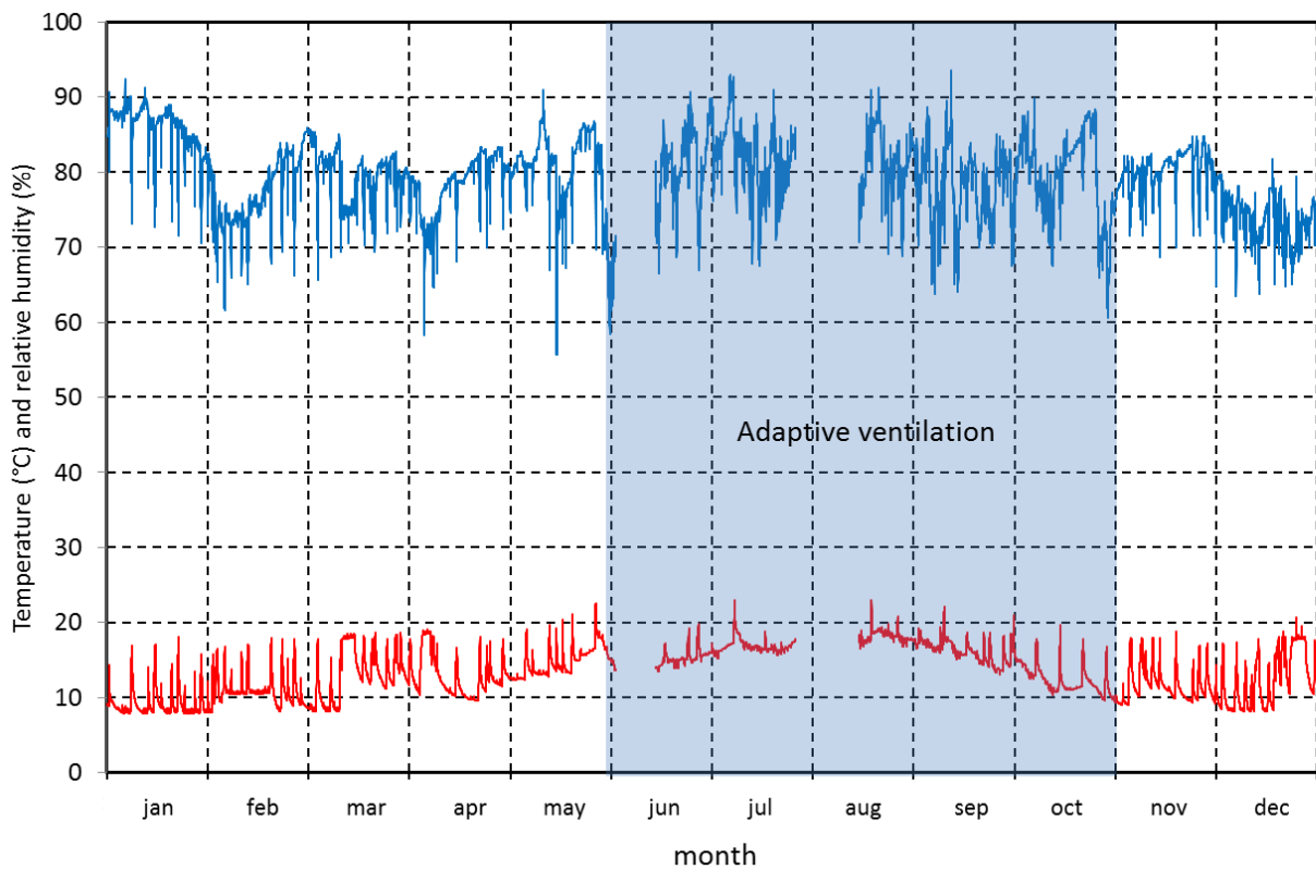
Figure 4 Climate record from Nødebo Church in 2012. Adaptive ventilation was operated from the beginning of June until the end of October, when background heating was started.
